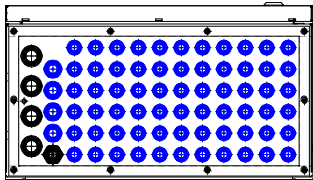
FLANGE VIEW
