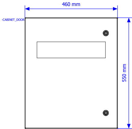
DOOR VIEW
