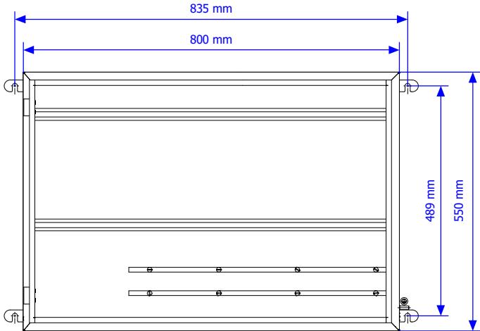
MOUNTING VIEW
