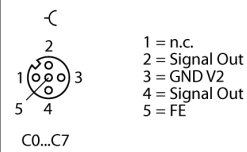
M12 × 1 Output
